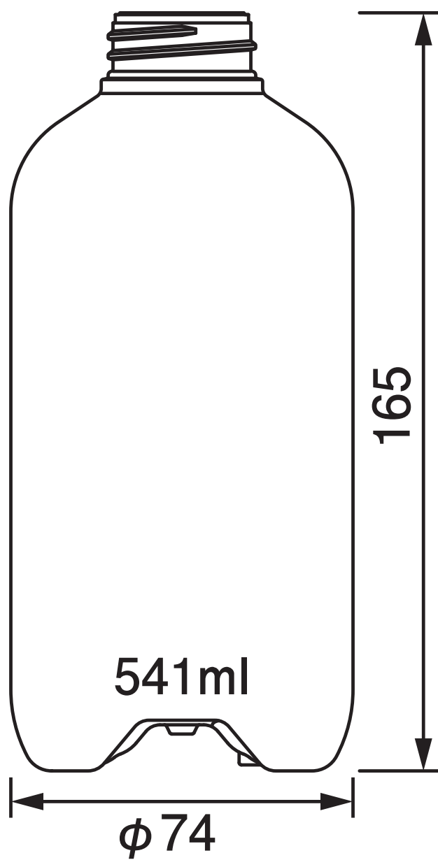
APD-500II (底上げ) APD-500II (Raised-base)
