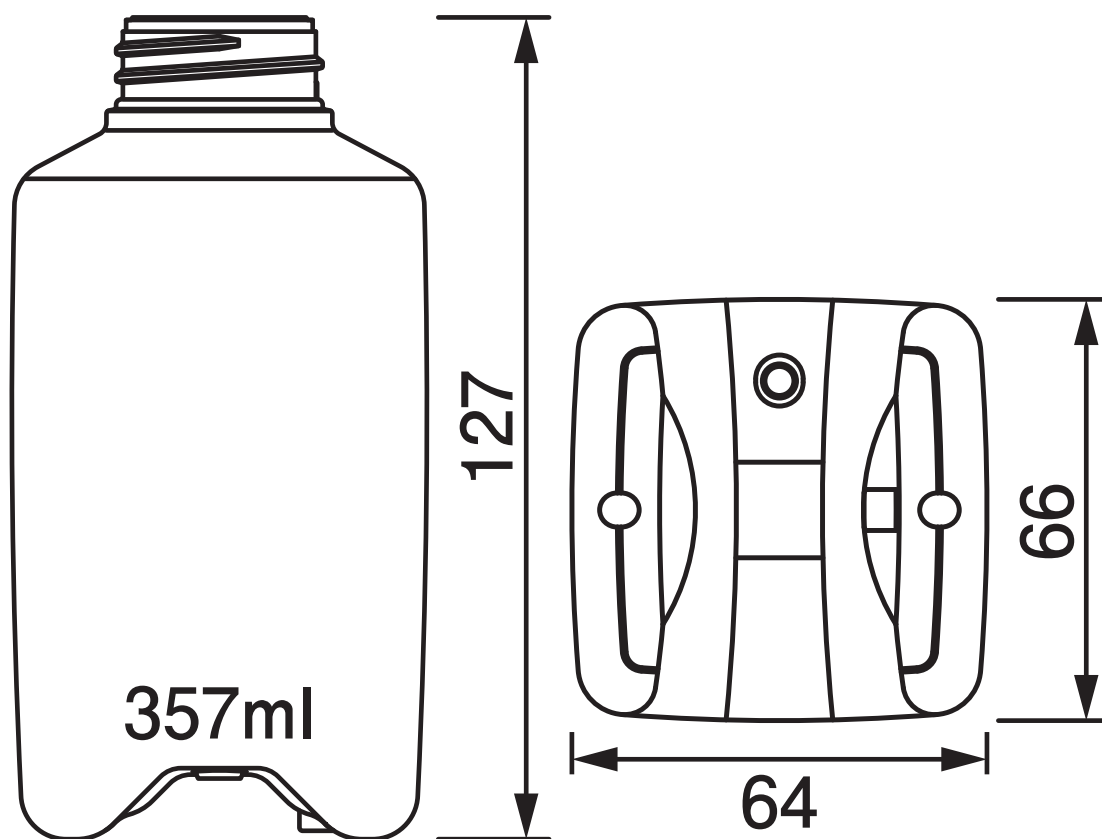
PBPD-300II (底上げ) PBPD-300II (Raised-base)
