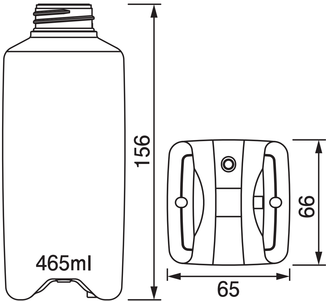
PBPD-400II (底上げ) PBPD-400II (Raised-base)
