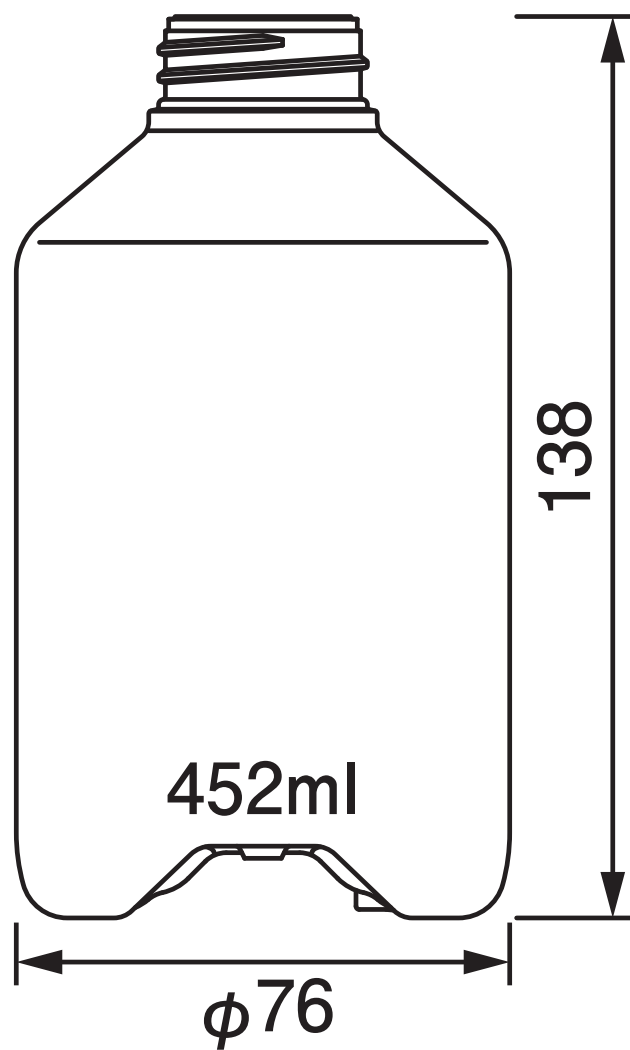
PMPD-400II (底上げ) PMPD-400II (Raised-base)
