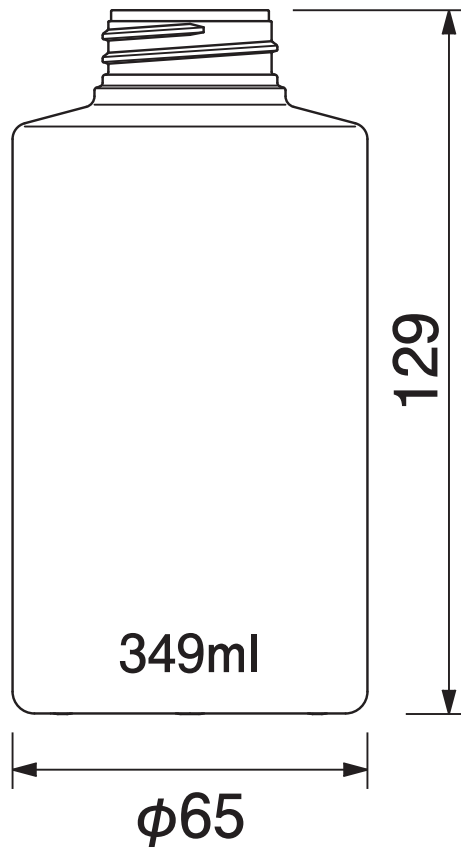
PEPI-300II(30.5G)
