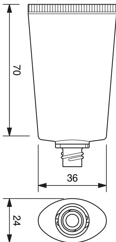
TN-30φオーバルチューブ -30.7 TN-30mm dia. Oval Tube-30.7
