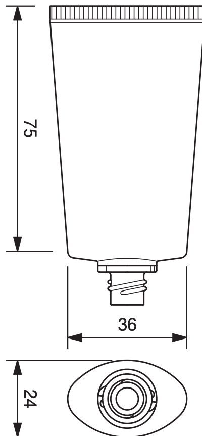
TN-30φオーバルチューブ -33.6 TN-30mm dia. Oval Tube-33.6
