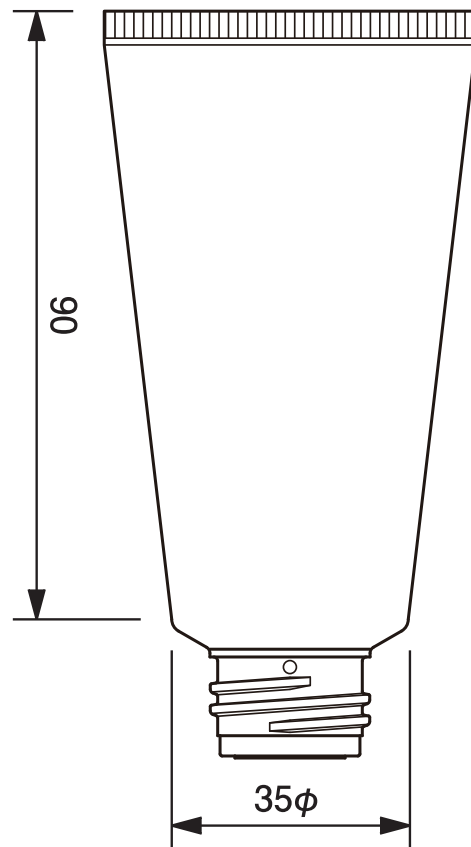
35φチューブ P口用 -61.5 35mm dia. P-Tube (for 24/410 Accessories)-61.5
