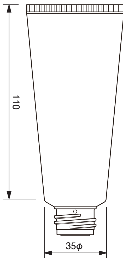
35φチューブ P 口用 -79.3 35mm dia. P-Tube (for 24/410 Accessories)-79.3
