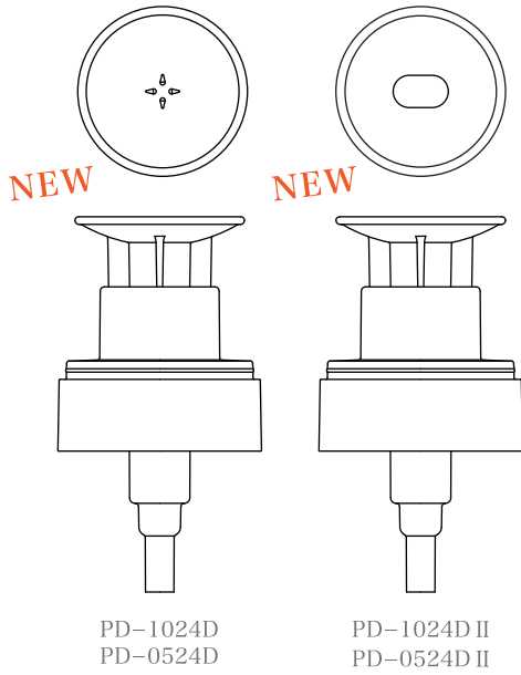
PD-24 Over Cap D Material: PP
